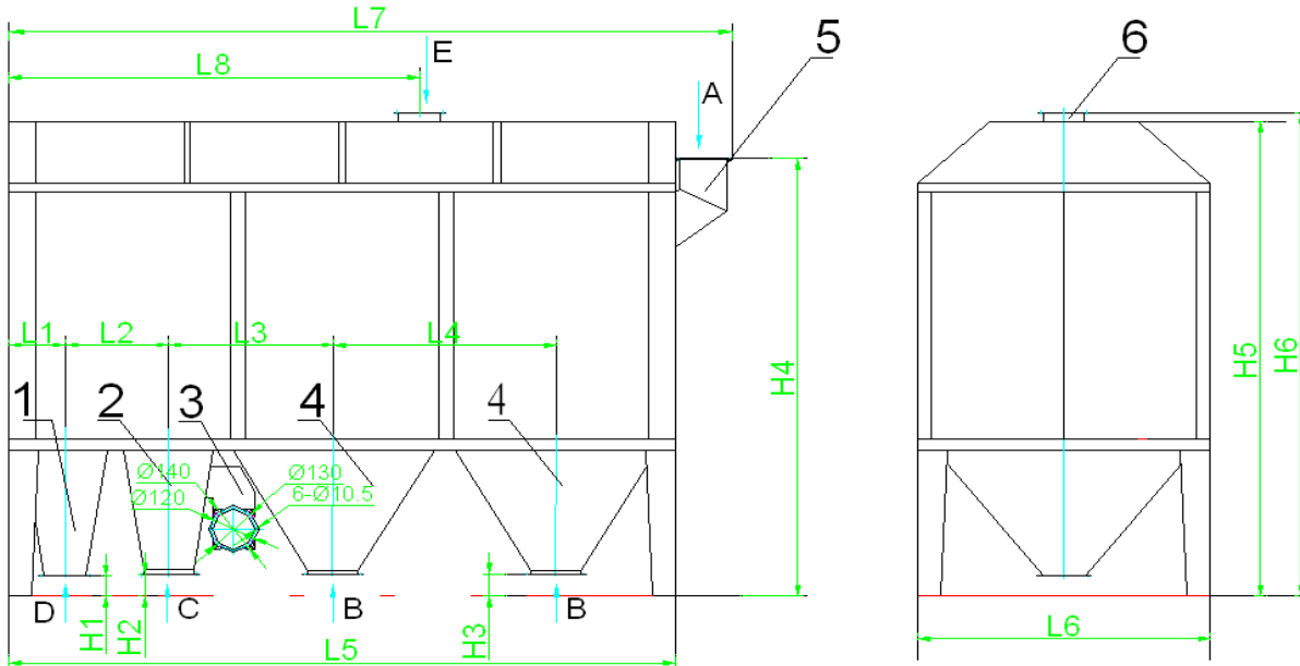
1.Outlet of large impurity 2.Grain Outlet 3.Bottom Air-intake Duct 4.Outlet of fine impurity 5.Grain Inlet 6.Top Air-intake Duct (Notes:LDDC85/190、100/200 have only one outlet of fine impurity ) Layout of LDDC Series Double-Deck Drum Pre-cleaner
