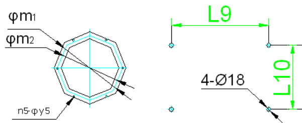
Inlet & outlet layout of LDDC series Double-Deck Drum Pre-cleaner
