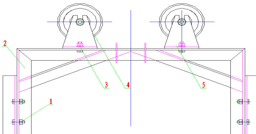
1. Lock nuts 2.Adjustable support 3.Roller lock nuts 4. Support roller 5. Roller support Layout of Screen Inclination Adjustment
